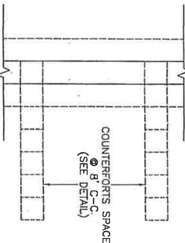
CONCRETE BLOCK RETAINING WALL DETAIL PLAN
